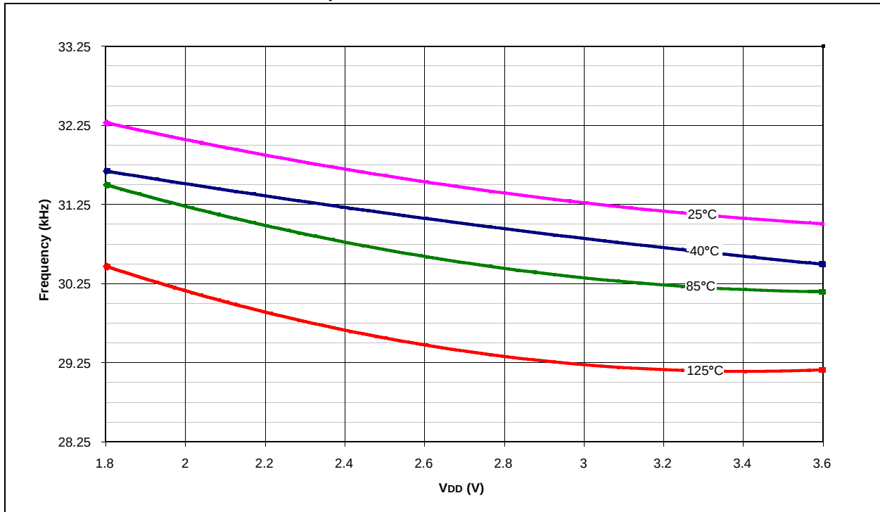
FIGURE 27-44: PIC18F4XK20/PIC18F2XK20 TYPICAL LF-INTOSC FREQUENCY (MAX./MIN. = 31.25 KHZ +/-15%)
