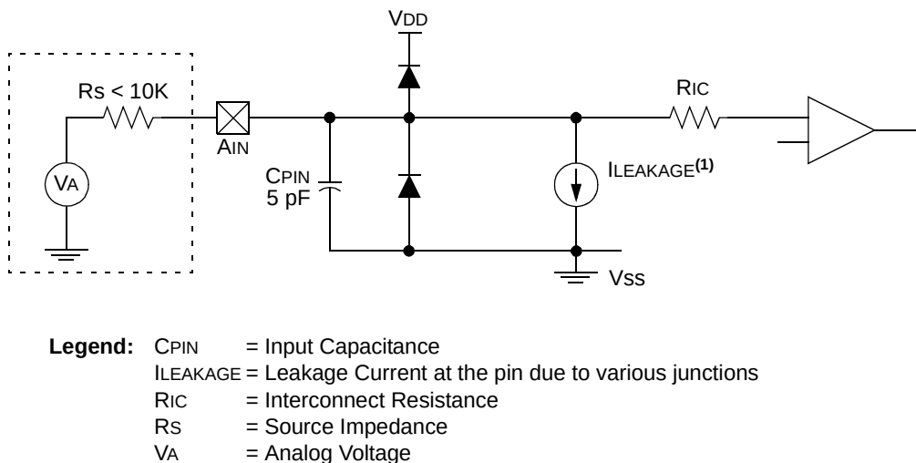
FIGURE 20-6: ANALOG INPUT MODEL
